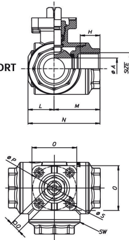
3-way ball valve, full bore with T-port .
