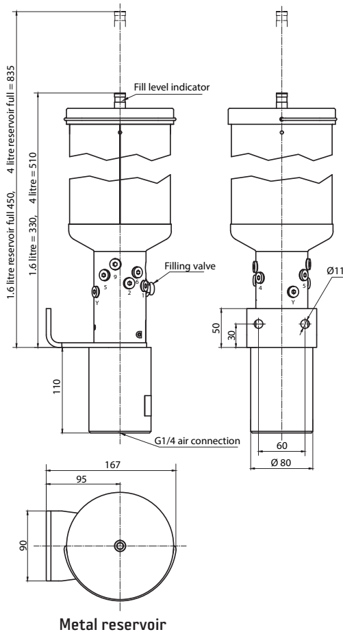
Metal reservoir
