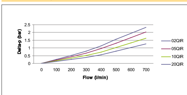
EPF Size 5 Length 1 Filter Elements with reverse flow valve
