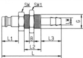
panel mount hose barb
