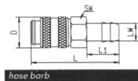
hose barb
