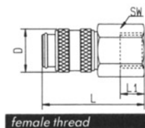
female thread
