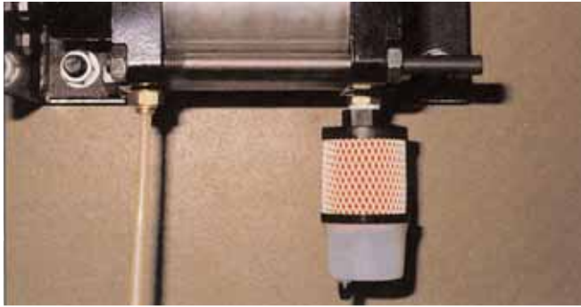
Air cylinders
